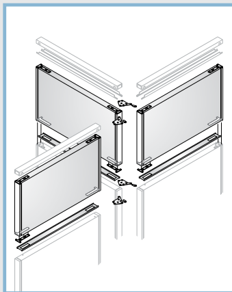
PolyStax "T" connection
