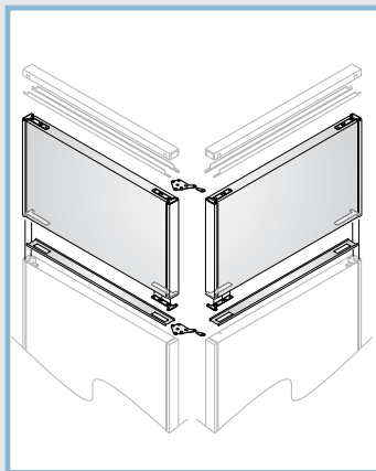
PolyStax "L" connection
