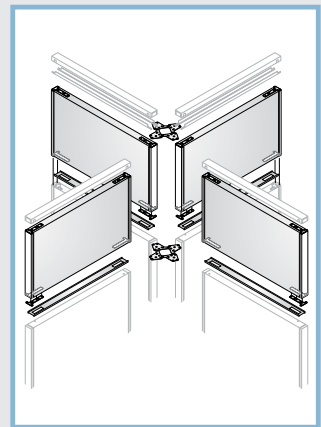
PolyStax "X" connection
